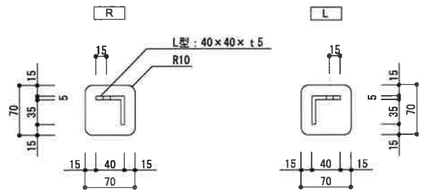
平面図S=1/5
