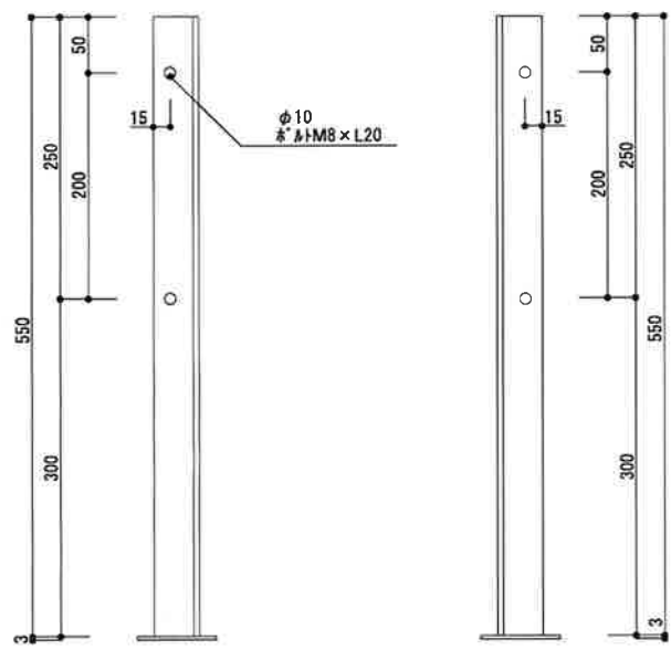
立面図S=1/5
